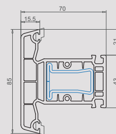
Traverse / Meneau 85 mm 102.288
