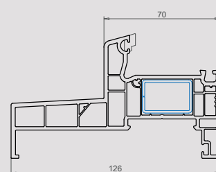
Dormant 74 x 126 mm Isolation de 120 mm 101.260
