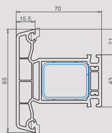
Traverse / Meneau 85 mm 102.287
