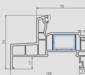
Dormant 74 x 106 mm Isolation de 100 mm 101.241
